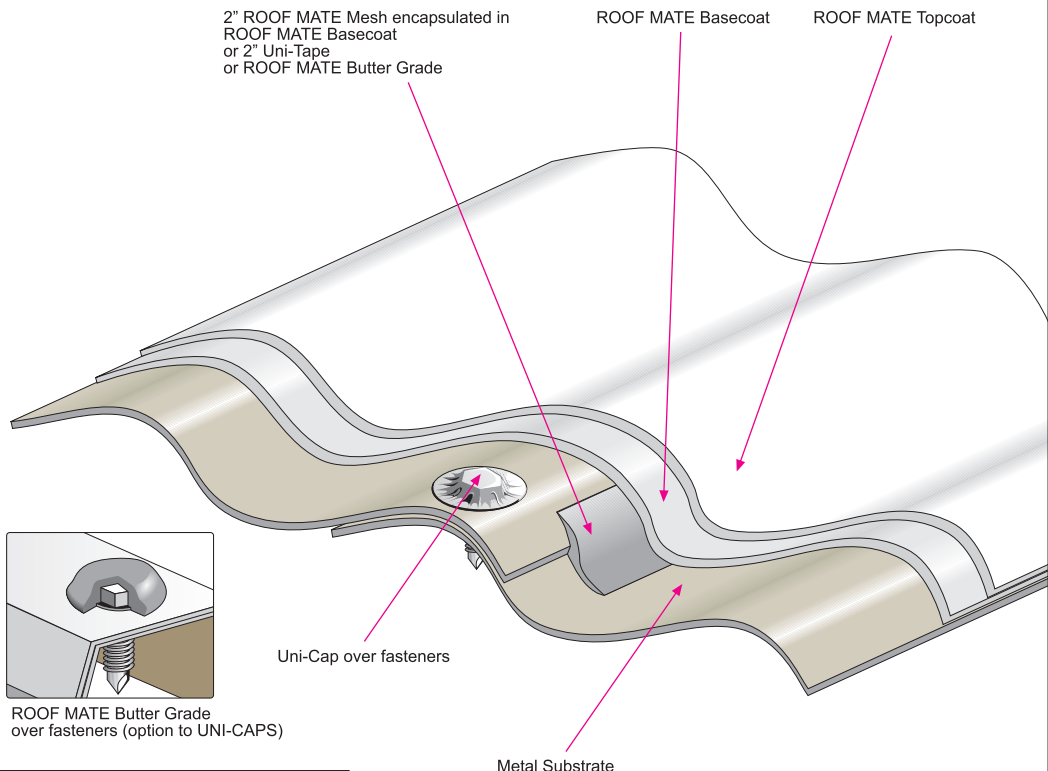
Title: ROOF MATE Corrugated Metal Vertical Side-Lap Seam Version: 01 Supersedes 04/18/06 Date: 06/14/07
