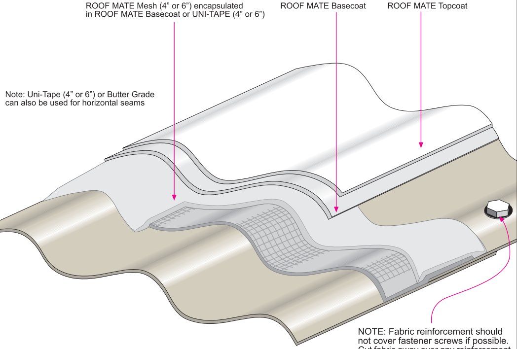
Title: ROOF MATE Corrugated Metal Horizontal End-Lap Seam Version: 01 Supersedes 04/18/06 Date: 06/14/07
