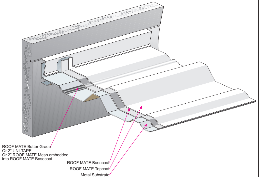
Title: ROOF MATE Concrete Parapet Termination w/ Counter-Flashing Version: 01 Supercedes 04/18/06 Date: 06/14/07
